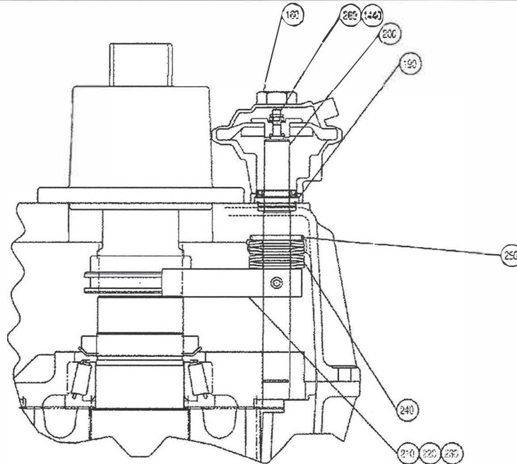
SECTION C-C
