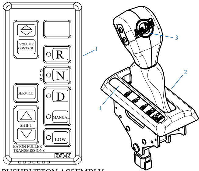
PUSHBUTTON ASSEMBLY COBRA LEVER - only for use with 10MY559M Mack Swing Arm Bracket
