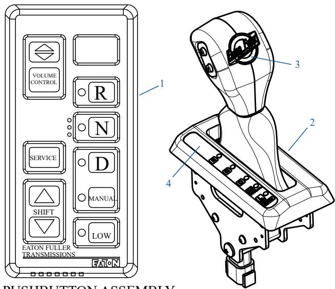
PUSHBUTTON ASSEMBLY
